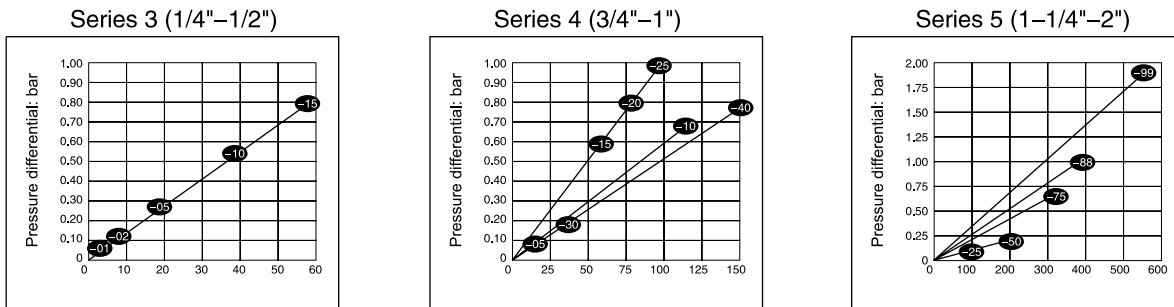
Pressure differential graphs categorised by size code
